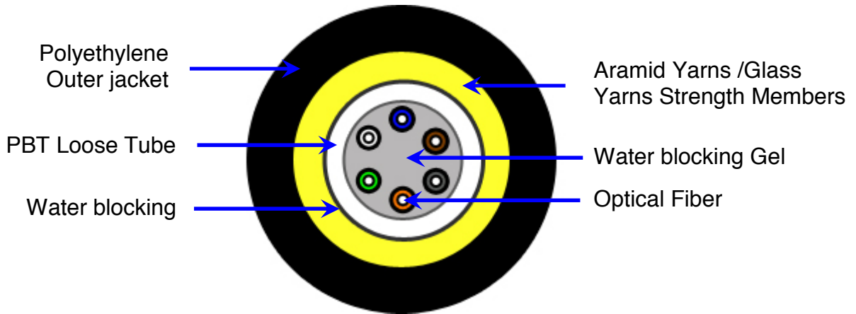
4-12 Fibers
